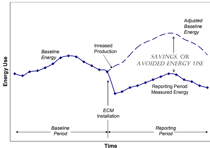
Figure 1 Example Energy History
